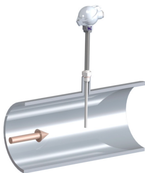
straight welded on piece
