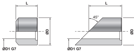
NV D Welded on piece for WT70 D
