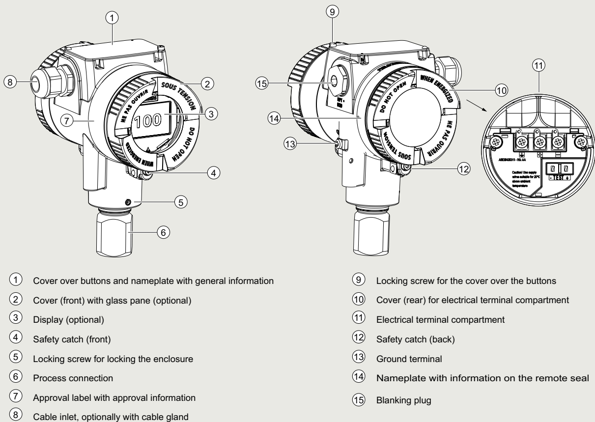
Device front view
