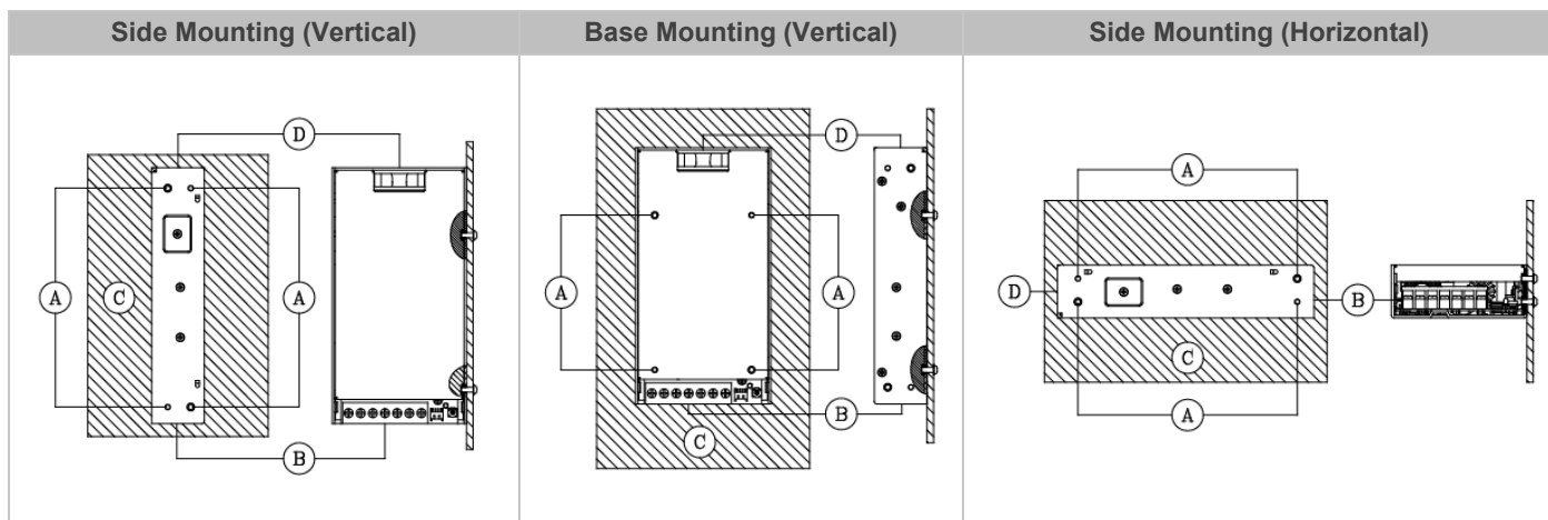
Fig. 2 Mounting Orientation
