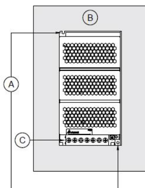
Fig. 2 Mounting Orientation
