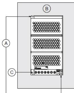
Fig. 2 Mounting Orientation
